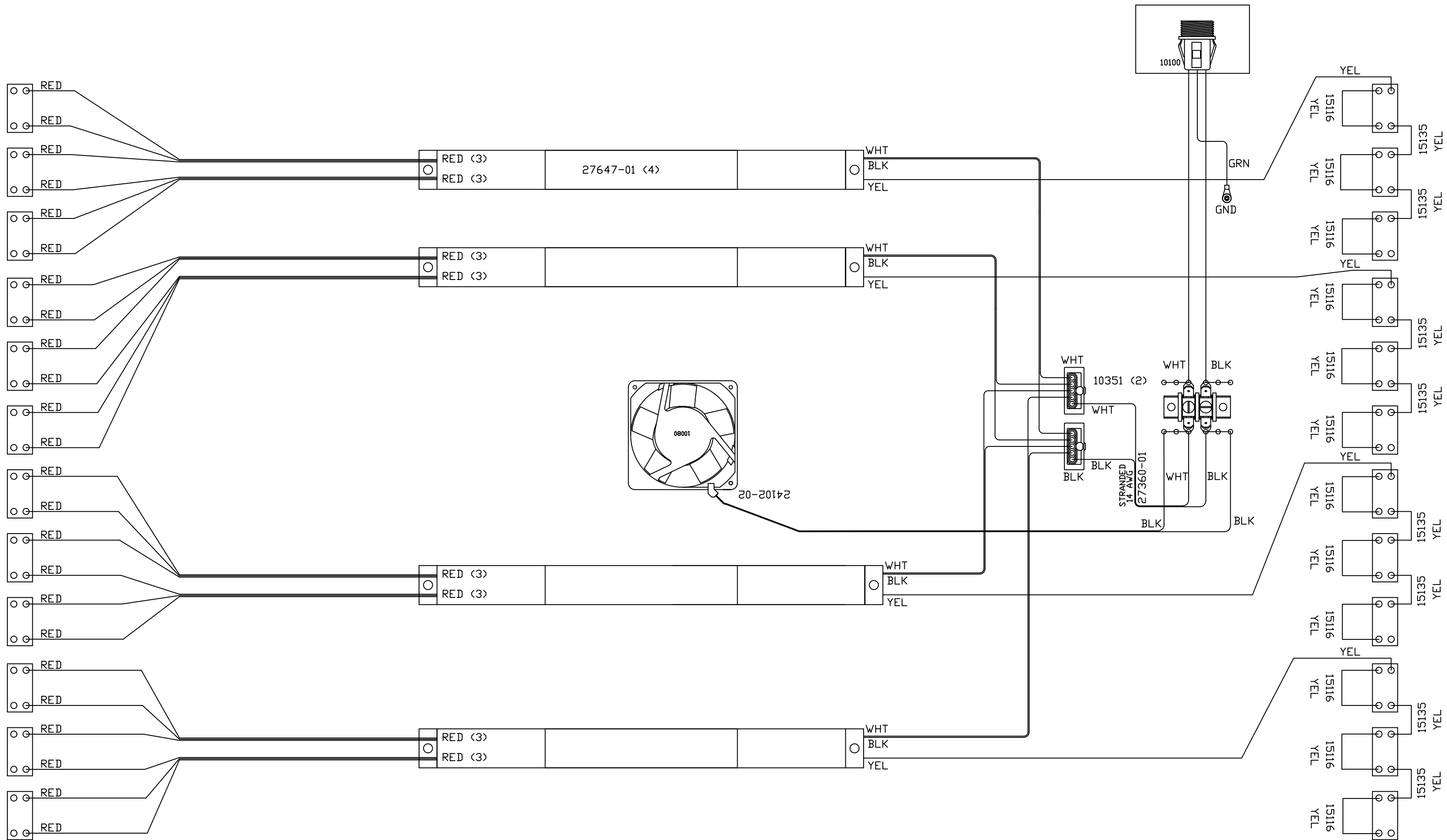
27520-01, REV A BENCH, 12 LAMP 120 VAC FRONT OF BED
